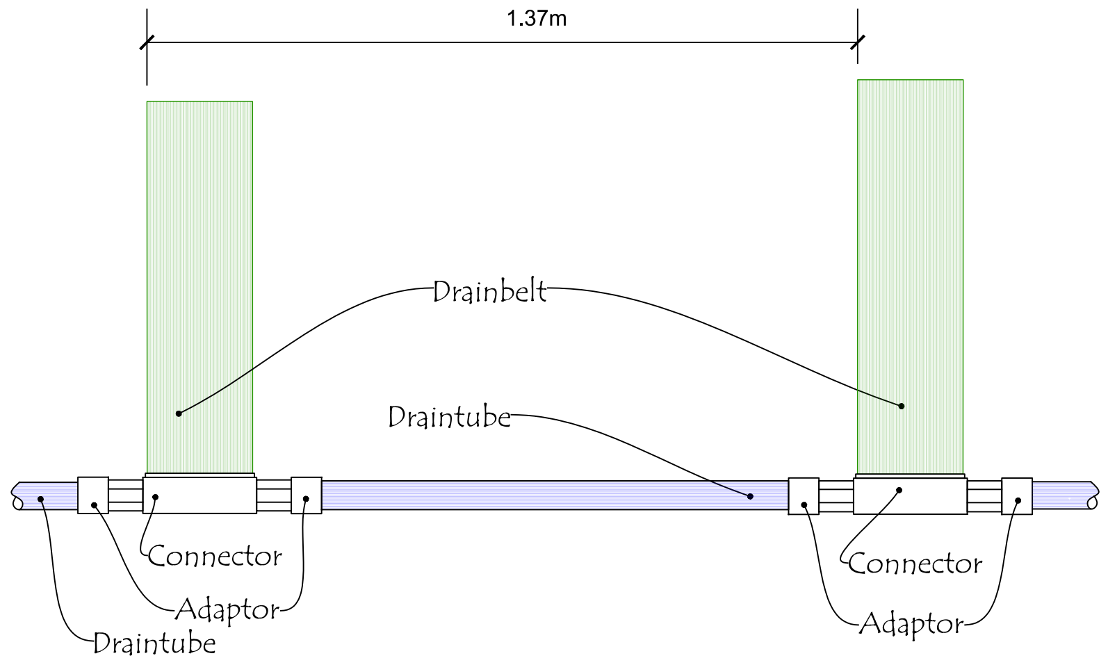
Front Elevation
